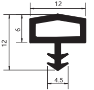
DW0001 Features: Material: aluminium + fire-resistant silicone Finish: anodised aluminium
