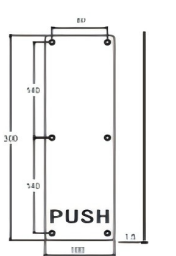
Push / pull plate| SP0007
