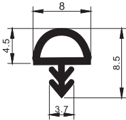
SE0005 Features: Material: fire-resistant silicone For dust, sound and thermal insulation
