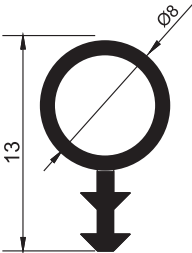
SE0003 Features: Material: fire-resistant silicone For dust, sound and thermal insulation
