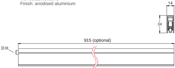
DW0002 Features: Material: aluminium + silicone Finish: anodised aluminium
