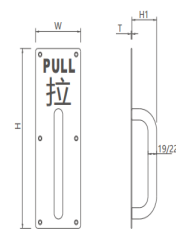
Push / pull plate| SP0002
