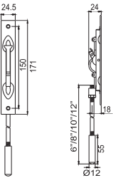
Flush bolt | DB0005 GB 12955: 90-minute fire certification Features: For double-leaf steel doors Material:304 stainless steel Finishes:SS/PSS/SB/PB
