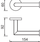
Robe hook | BA0704
