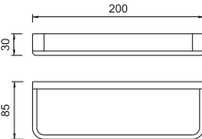
Toilet roll holder | BA0903
