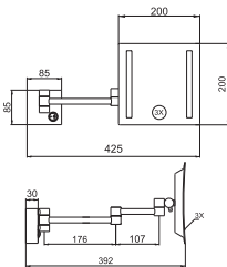
Magnifying mirror | MR0202 Features Materials: brass and zinc alloy Finish: CP Wall-mounted extendable LED mirror, 3x-5x magnification
