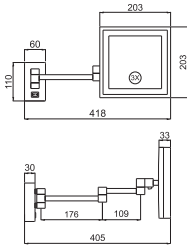
Magnifying mirror | MR0201 Features Materials: brass and zinc alloy Finish: CP Wall-mounted extendable LED mirror, 3x-5x magnification
