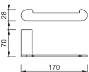
Robe hook | BA0604
